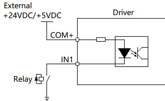
Figure 2-3 single-ended input
