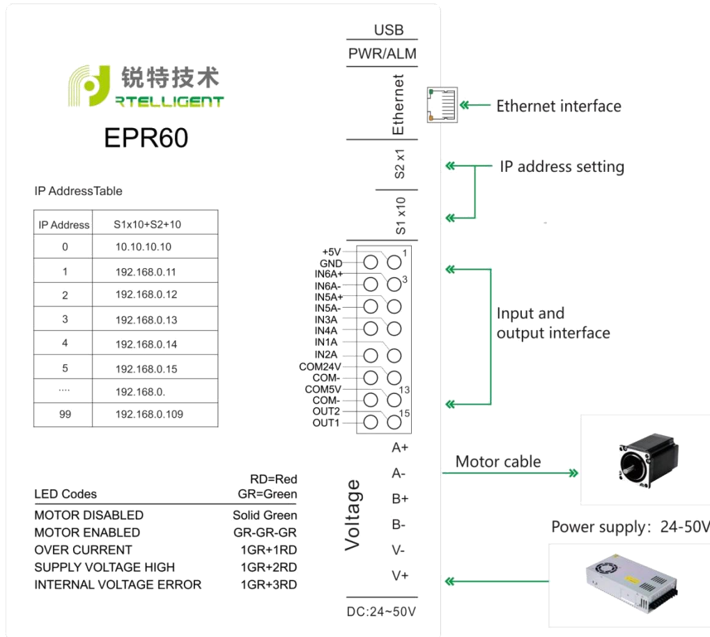
Figure 2-1 Hardware diagram
