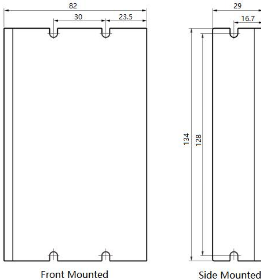
Figure 2-9 Drive dimensions
